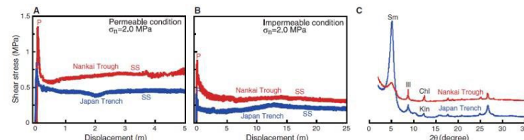
Fig. 3. Comparison of experimental results for decollement materials of the Japan Trench and the Nankai Trough. Shear stress measured during high-velocity shearing under permeable (A) and impermeable (B) conditions at \sigma_n of 2.0 MPa, plotted as a function of displacement. P, initial peak shear stress; SS, steady-state shear stress. (C) X-ray diffraction patterns for the decollement materials from the Japan Trench and the Nankai Trough, obtained for the <math>2\theta</math> fractions in the ethylene-glycolated state. Sm, smectite; Ill, illite; Chl, chlorite; Kln, kaolinite.
