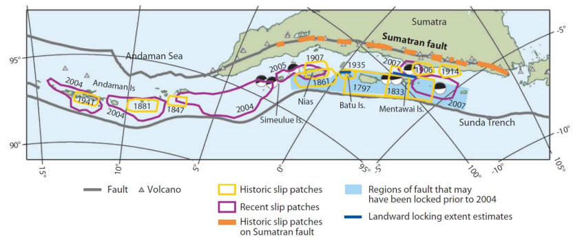
Figure 10 Map of the Sunda margin showing approximate regions of coseismic slip and regions where the subduction fault may have been locked prior to 2004. Slip patches are labeled by year of earthquake occurrence. Regions of fault that may have been locked prior to 2004 are compiled from Prawirodirdjo et al. (1997) and McCaffrey (2002). Landward (down-dip) locking extent estimates (thick blue lines) are from Zachariassen et al. (1999) and Natawidjaja et al. (2007) for the Mentawai Islands region and from Natawidjaja et al. (2004) for the Batu Islands region. Earthquake slip sources: 1847, 1881, and 1947 Andaman from Bilham et al. (2005); 1861, 1906, 1907, and 1914 Sumatran forearc from Newcomb & McCann (1987); 1797 and 1833 from Natawidjaja et al. (2006); 2004 slip from Subarya et al. (2006); 2005 slip from Briggs et al. (2006); 2007 slip from USGS seismological slip models at http://earthquake.usgs.gov/regional/world/historical.php . Historic slip patches on the Sumatran fault are from Sorensen (2008).
