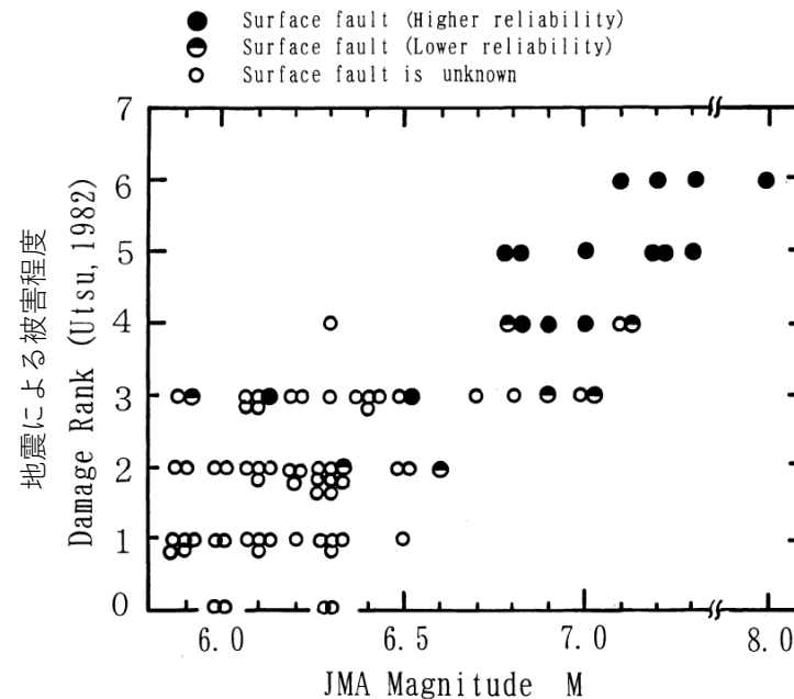
Fig. 9. Relation between damage rank and JMA magnitude M . Solid circles indicate the events accompanying surface faults of higher reliability marked with (H) in Table 2, and half solid circles indicate the events accompanying surface faults of lower reliability marked with (L) or * in Table 2. Open circles indicate the events for which any surface fault (including closely related active fault) is not found.
