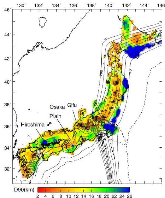
Fig. 4. Distribution of D90's, volcanoes, and M > 6.5 earthquakes. D90's are shown by the color scale at the bottom. Regions with the number of events insufficient for the lower threshold are shaded white. Active and Quaternary volcanoes are shown by triangles. Large open circles represent large earthquakes ( M > 6.5 ) that occurred in the period from 1926–2010. Depth to the upper surface of the subducting Pacific and Philippine Sea plates is shown by contours. Depth to the subducting plates is from Baba et al. (2002), Nakajima and Hasegawa (2007), Hirose et al. (2008), Nakajima et al. (2009), and Kita et al. (2010).
