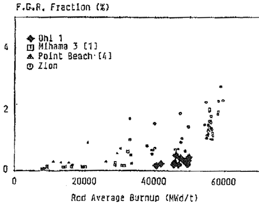
Figure 6 Fission Gas Release Data
