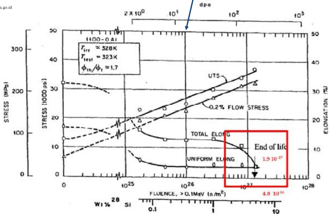
Figure 5. Fluence dependence of tensile properties of Aluminum [35]
