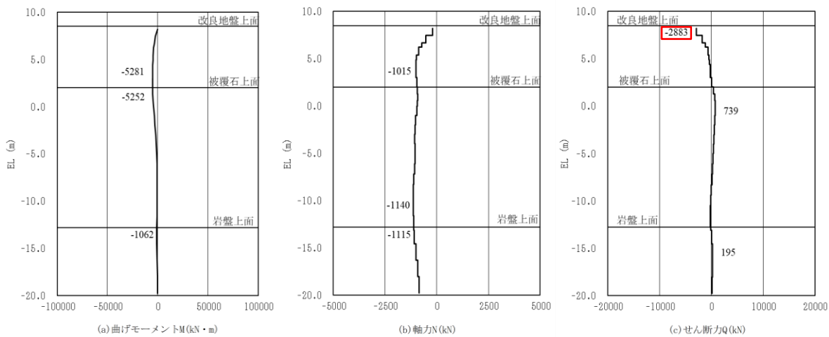
④-④断面, 陸側杭, S d - D ( + + ), t=9.13s
