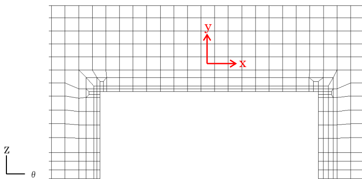
遮蔽壁（本体）拡大
