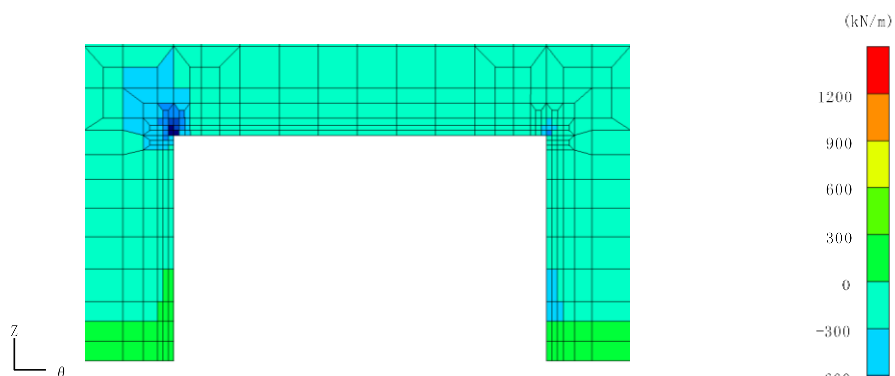
遮蔽壁（本体）拡大
