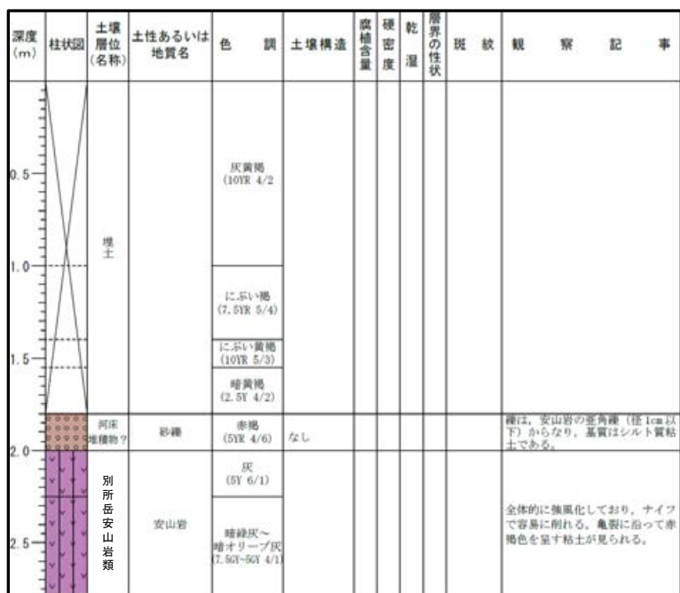
柱状図b
