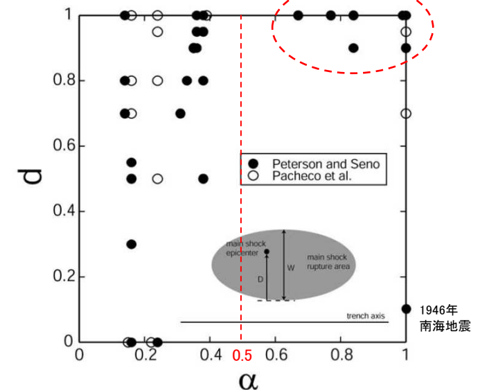
Fig. 1. The relative hypocentral depth d versus the seismic coupling coefficient α obtained for large interplate earthquakes at subduction zones (Table 1). Solid and open circles stand for α values from Peterson and Seno [7] and from Pacheco et al. [15], respectively. When α is estimated to be greater than 1 (Table 1), it is reduced to 1. The relative hypocentral depth d is defined by D / W , where D is the distance from the trenchward edge of the rupture area to the epicenter and W is the width of the rupture area in the direction perpendicular to the trench axis (inset).
