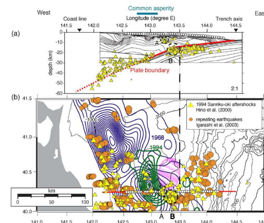
Fig. 5. (a) Model with iso-velocity contours as for Fig. 3a, superimposed on focal depths of aftershocks of the 1994 earthquake [10] projected onto the vertical cross section off-eastern Aomori forearc region. The horizontal axis indicated in the upper part shows the east longitude ( ^{\circ} E) corresponding to the position of our profile, and vertical axis is depth below sea level (km). Yellow triangles show focal depths of the 1994 aftershocks. Black dashed circles labeled A and B denote clusters of aftershocks discussed in the text. The red thick line and the black thick vertical dashed line mark location of the plate boundary and the location of the binding point revealed by this study, respectively. The blue bar in the upper part shows the location of common asperity of the 1968 and the 1994 earthquakes, from Nagai et al. [4]. Open circles are OBS deployment positions. Vertical exaggeration is 2 times. (b) Spatial distribution of repeating earthquakes from Igarashi et al. [28]. Orange circles show the repeating earthquakes for the period from April 1992 to July 2000 ( M \geq 3 or larger). The red line indicates the location of the seismic refraction profile and white circles are OBS locations for this study. Blue and green contours denote the large moment release areas, as in Fig. 1 [4]. Seafloor topography is contoured at 500-m intervals.
