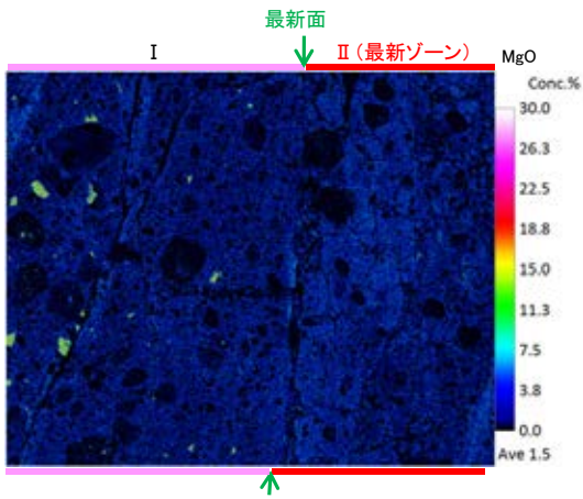
MgO
