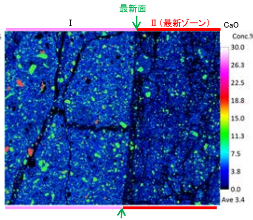
CaO
