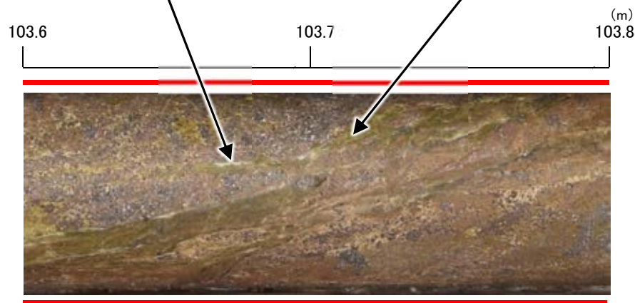
拡大写真(H-1.1孔 103.6~103.8m)
