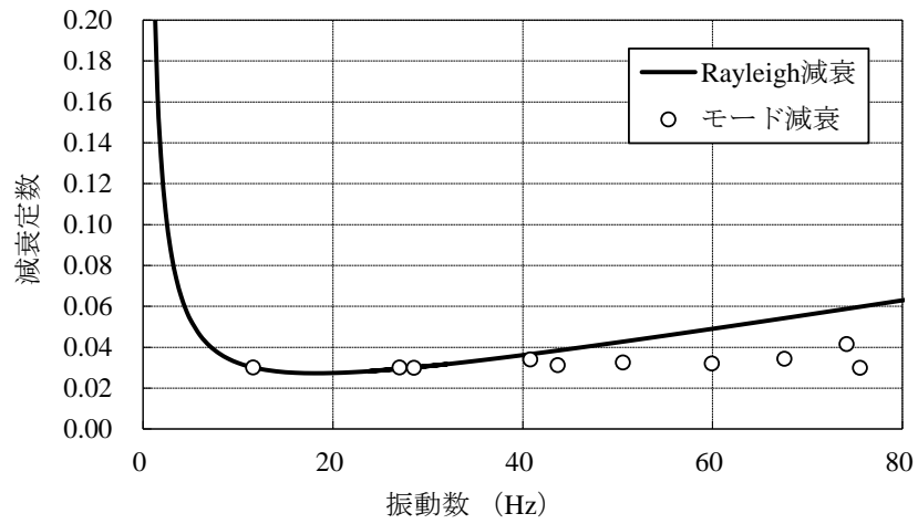
(Rayleigh 減衰)
