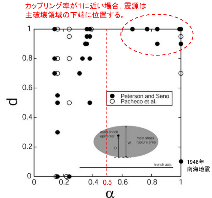
Fig. 1. The relative hypocentral depth d versus the seismic coupling coefficient \alpha obtained for large interplate earthquakes at subduction zones (Table 1). Solid and open circles stand for \alpha values from Peterson and Seno [7] and from Pacheco et al. [15], respectively. When \alpha is estimated to be greater than 1 (Table 1), it is reduced to 1. The relative hypocentral depth d is defined by D/W , where D is the distance from the trenchward edge of the rupture area to the epicenter and W is the width of the rupture area in the direction perpendicular to the trench axis (inset).
