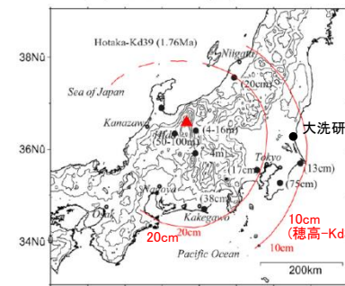
(12) Distribution of Hotaka-Kd39 tephra
