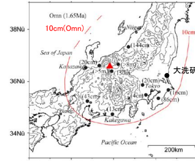
(14) Distribution of Omine tephra
