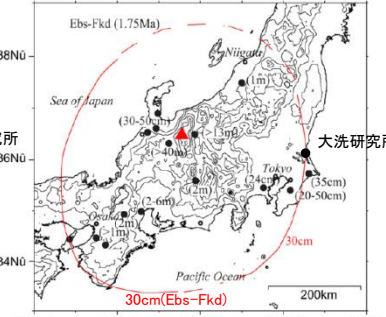
(13) Distribution of Ebisutoge-Fukuda tephra
