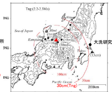
(9) Distribution of Taniguchi-Tsp tephra
