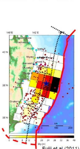
Fujii et al.(2011)
