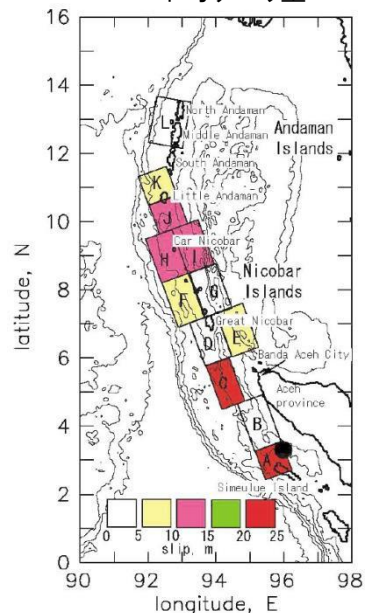
(Tanioka et al. (2006))
