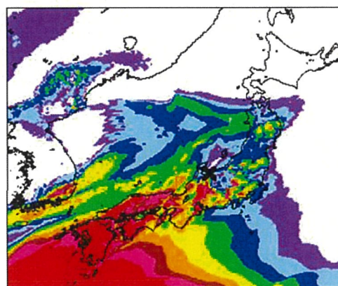
Convective Available Potential Energy (Max) [J/kg] 200 400 600 800 1000 1200 1400 1600 1800
