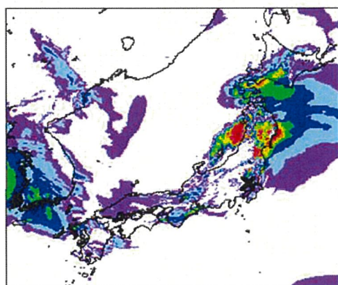
Storm Relative Helicity [ m^2/s^2 ] 100 150 200 250 300 350 400 450 500
