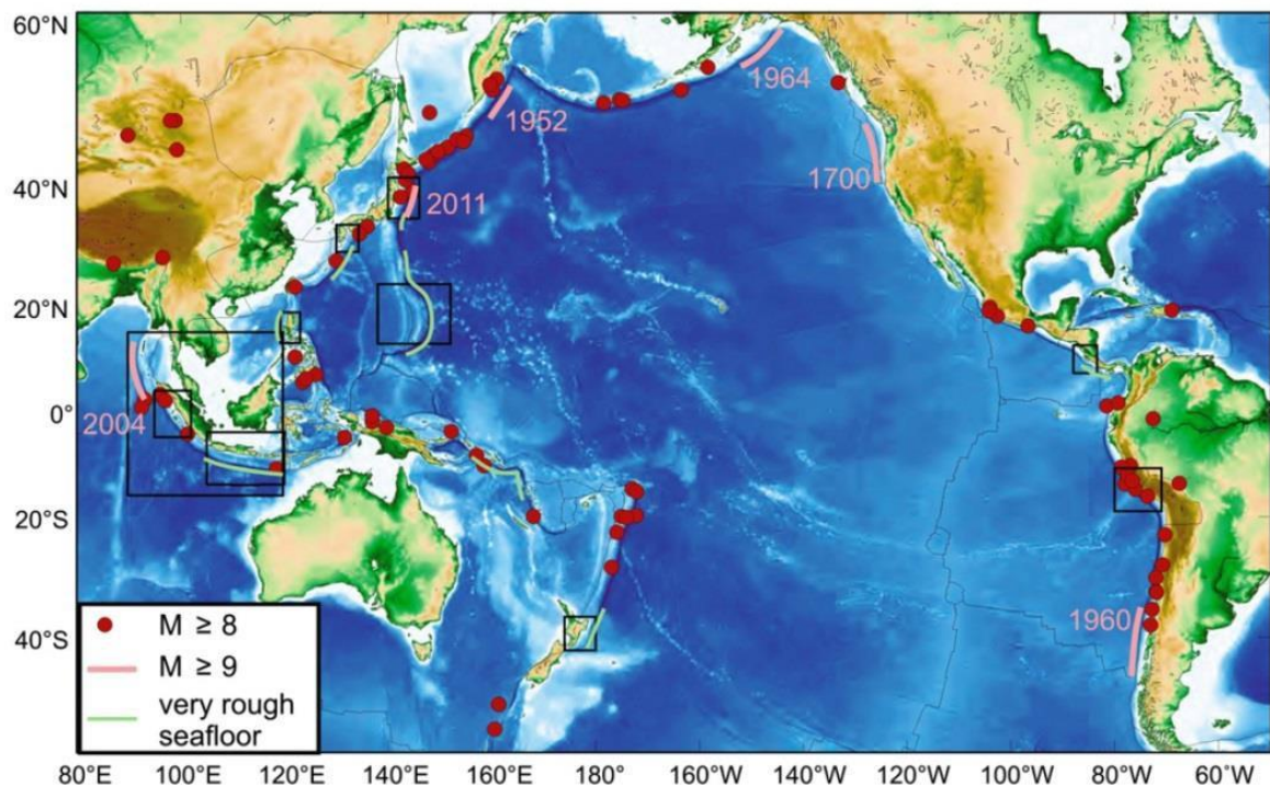
Fig. 1. World map showing general lack of correlation between rugged subducting seafloor and great megathrust earthquakes and showing locations of map areas of Fig. 2 through 10 and 14. Rupture extents of giant ( M_w \geq 9 ) events are indicated with pink lines. Epicentre locations of other great ( M_w \geq 8 ) events are from the USGS/NOAA catalogue for the time period of 1903–2012.
