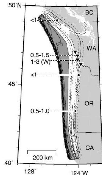
a Long-Narrow M w 9.0
