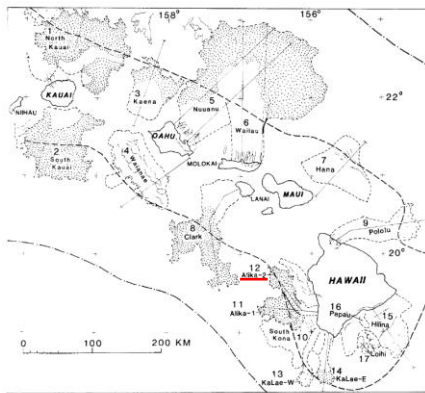
Fig. 3. Map of southeastern Hawaiian Ridge showing major faults bounded by dashed lines identified by number in text and Table 1; compare with Figure 1. Dotted area, hornedocks ground (wavy spaced where subside); hatched lines, scarp; thin down-slope directed lines, submarine canyon and line; substantial counterparts; heavy dashed line, axis of the Hawaiian Trench; dash-dotted line, crest of the Hawaiian Arch.
