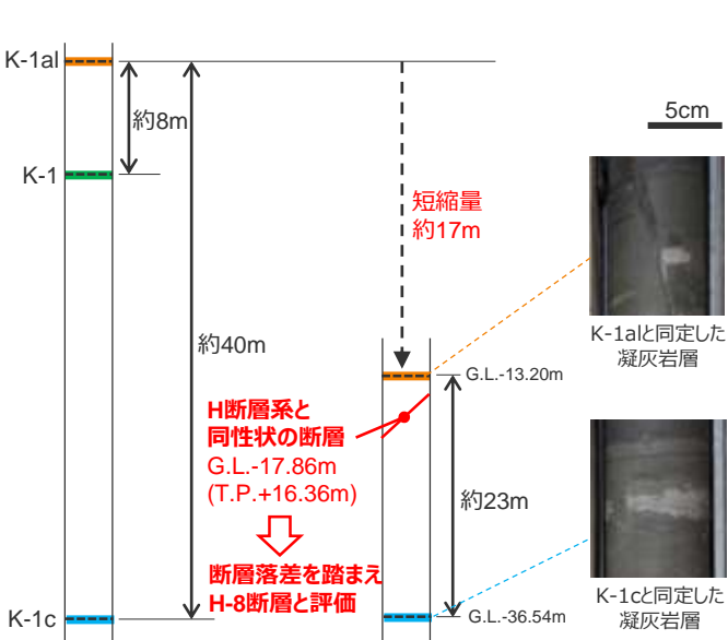
敷地内で確認される凝灰岩の層厚 (Ash layer thickness confirmed on-site) D-2孔の簡易柱状図 (Simplified columnar diagram of D-2 hole) D-2孔コア写真 (D-2 hole core photo)
