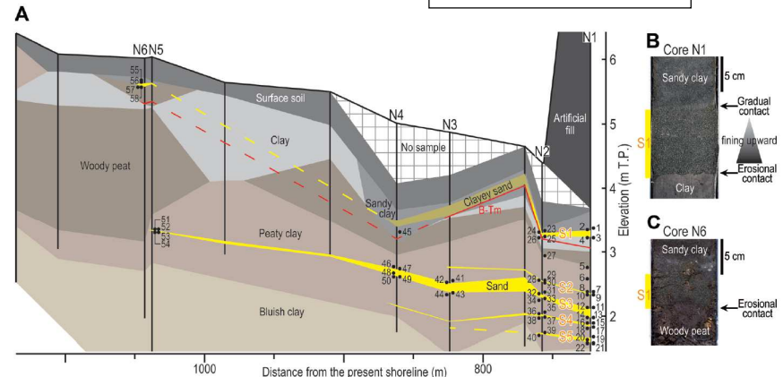
Figure 3. (A) Cross-section of the study area along the transect shown in Fig. 1C. Circles numbered 1-58 correspond to the radiocarbon ages listed in Table 2. Elevations are relative to mean sea level in Tokyo Bay (Tokyo Peil: T.P.). Photographs of S1 in core N1 (B) and core N6 (C). This figure is available in colour online at wileyonlinelibrary.com.
