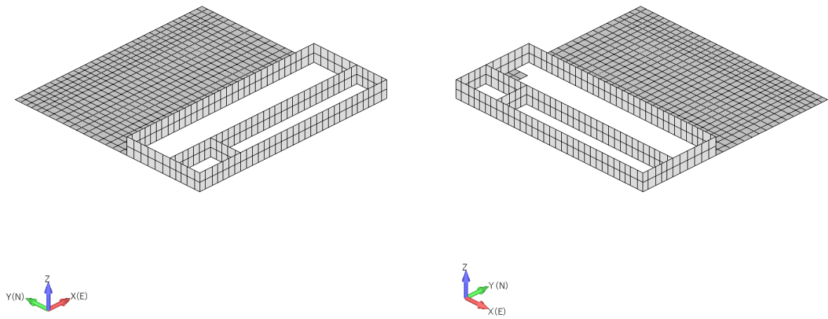
(b) T.M.S.L. 70.20m ~ T.M.S.L. 77.50m
