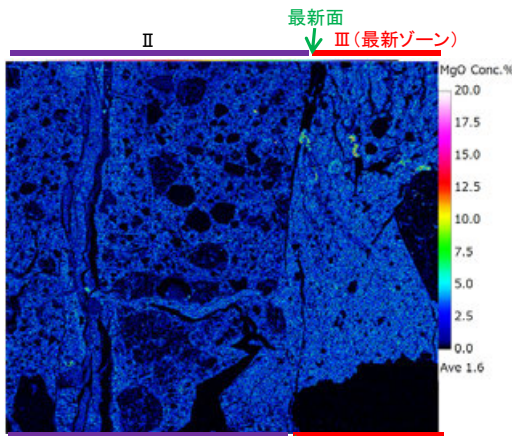
MgO
