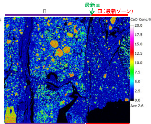
CaO
