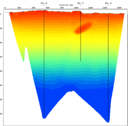
velocity (m/sec)
