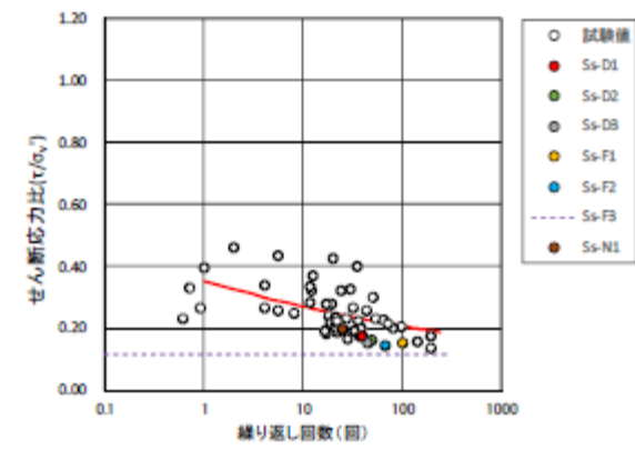
(a) 粘土
