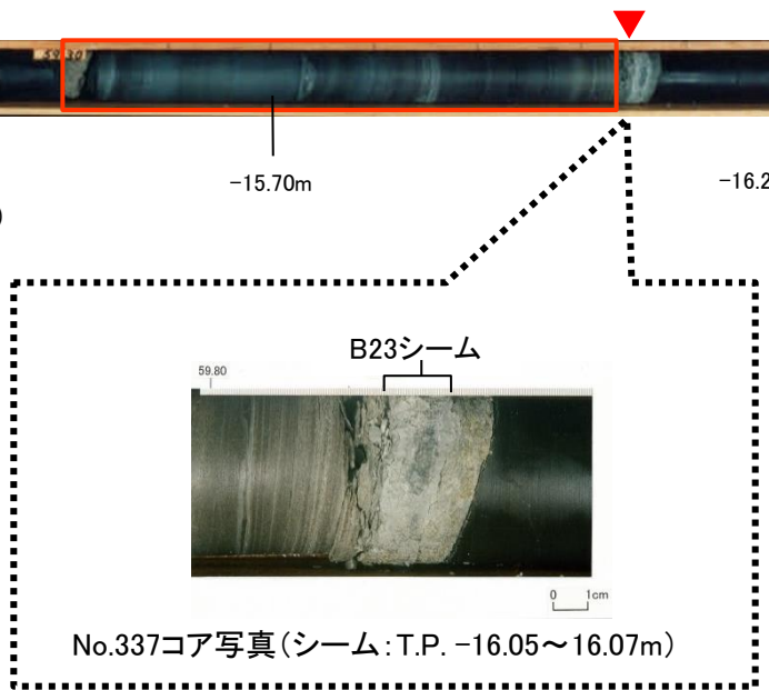
No.337コア写真 (T.P.-14.20~16.20m)
