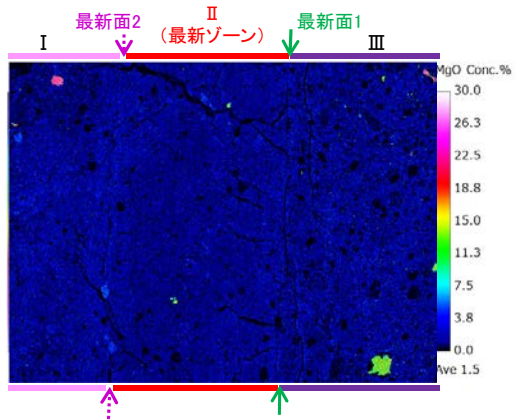
MgO
