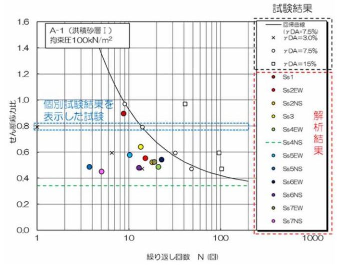
(a) 拘束圧100kN/m 2
