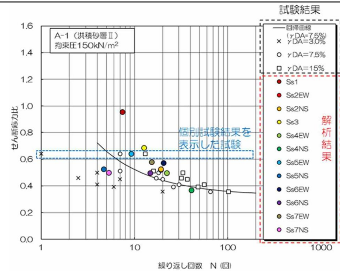
(a) 拘束圧150kN/m 2
