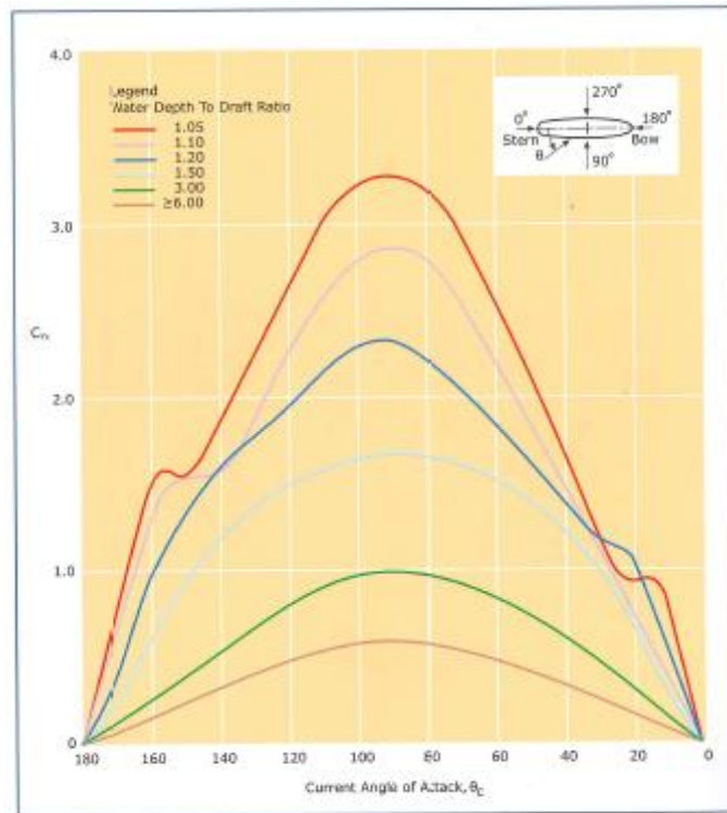
Figure A10: Lateral Current Drag Force Coefficient ( C_y ) - Loaded Tanker
